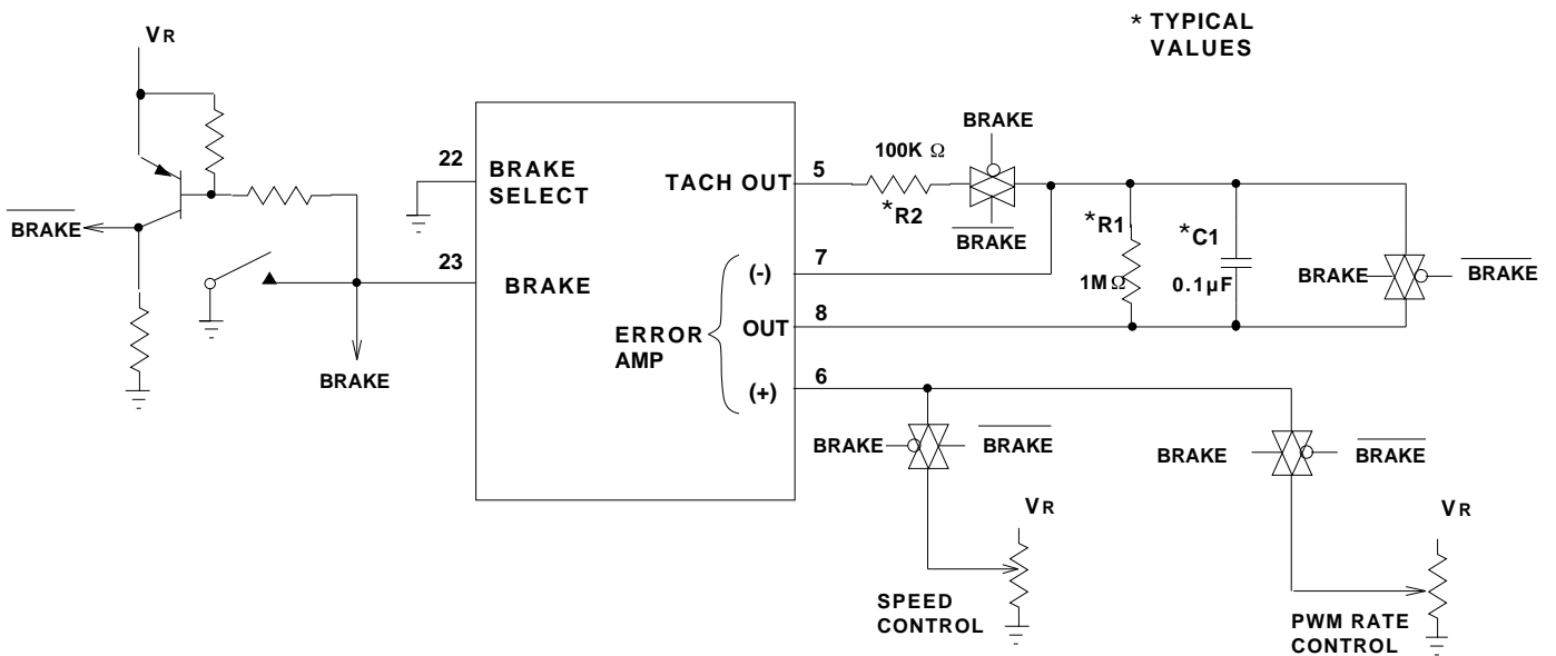
FIGURE 8. PWM BRAKING
