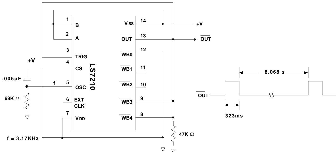
FIGURE 6. ASYMMETRICAL FLASHER
